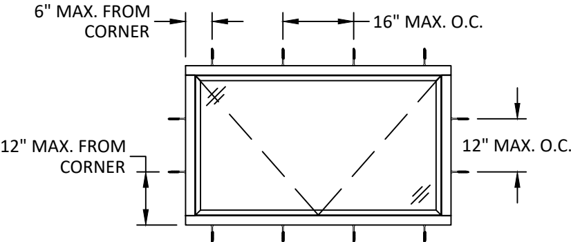
ANCHOR LAYOUT
